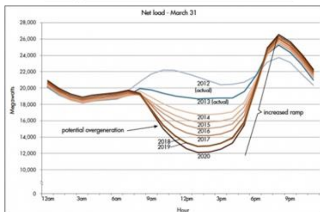
Figure 1: California's Duck Curve Chart
