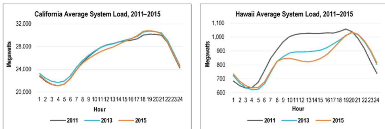
Figure 7: California and Hawaii Average System Load, 2011–2015
