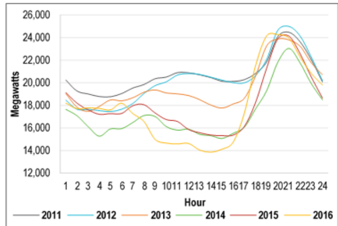
Figure 2: Lowest March Daytime Net Load, 2011–2016
