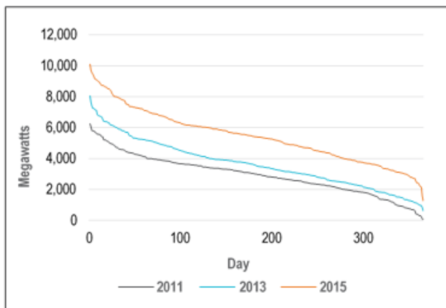
Figure 4: Daily Late-Day Three-Hour Ramp, 2011–2015
