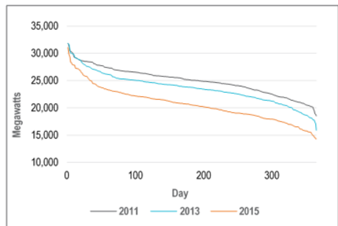
Figure 3: Daily Daytime Minimum Net Load, 2011–2015
